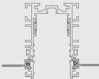
Invia flush recessed profile
